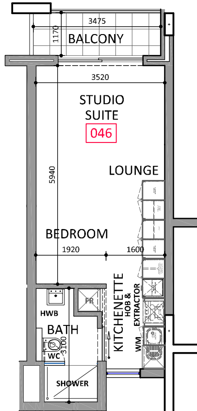
UNIT 046 FIRST PLAN LAYOUT - Scale 1:100
