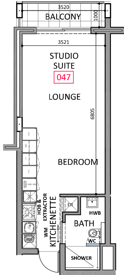
UNIT 047 FIRST PLAN LAYOUT - Scale 1:100
