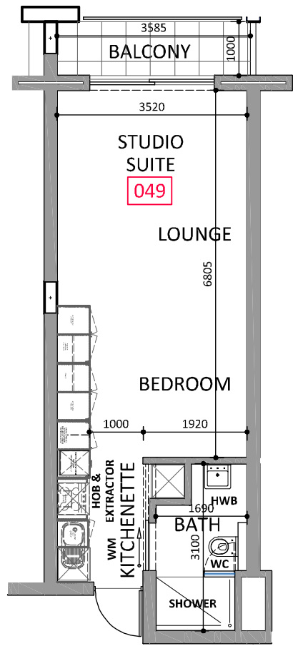
UNIT 049 FIRST PLAN LAYOUT - Scale 1:100
