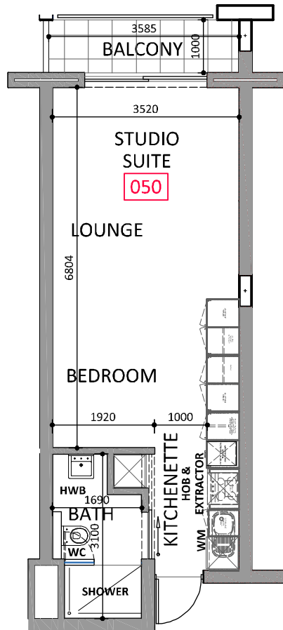
UNIT 050 FIRST PLAN LAYOUT - Scale 1:100
