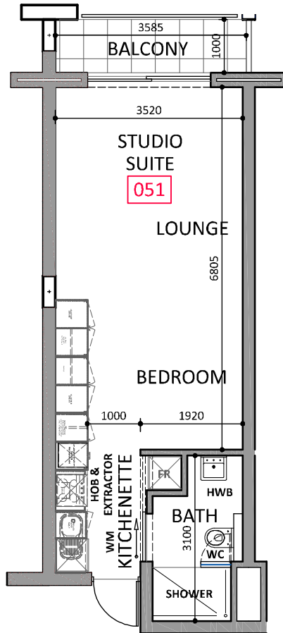
UNIT 051 FIRST PLAN LAYOUT - Scale 1:100
