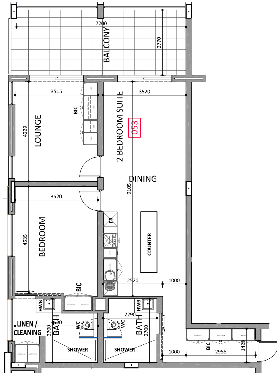
UNIT 053 FIRST PLAN LAYOUT - Scale 1:100
