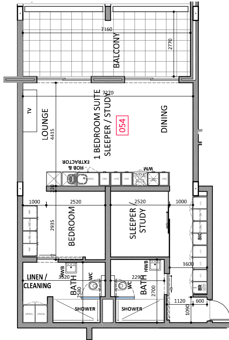
UNIT 054 FIRST PLAN LAYOUT - Scale 1:100
