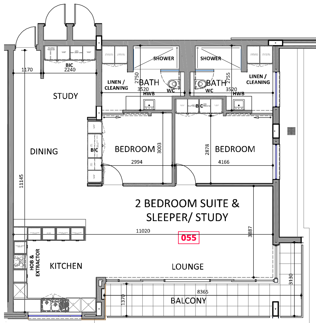
UNIT 055 FIRST PLAN LAYOUT - Scale 1:100
