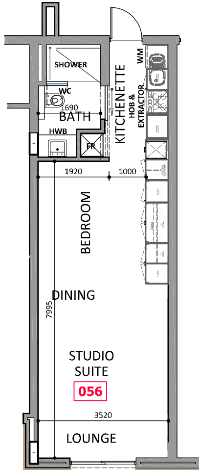
UNIT 056 FIRST PLAN LAYOUT - Scale 1:100
