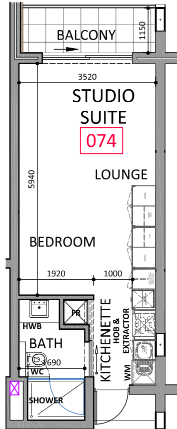
UNIT 074 SECOND PLAN LAYOUT - Scale 1:100
