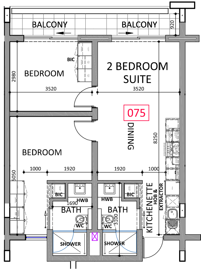
UNIT 075 SECOND PLAN LAYOUT - Scale 1:100
