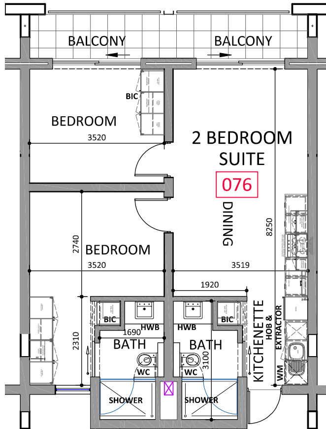
UNIT 076 SECOND PLAN LAYOUT - Scale 1:100
