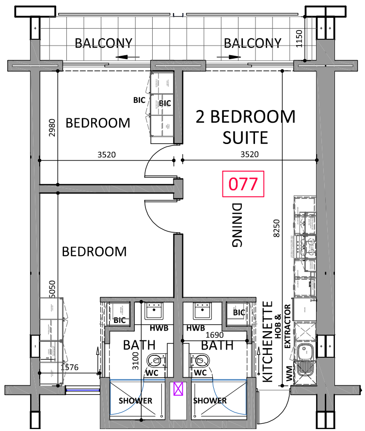
UNIT 077 SECOND PLAN LAYOUT - Scale 1:100
