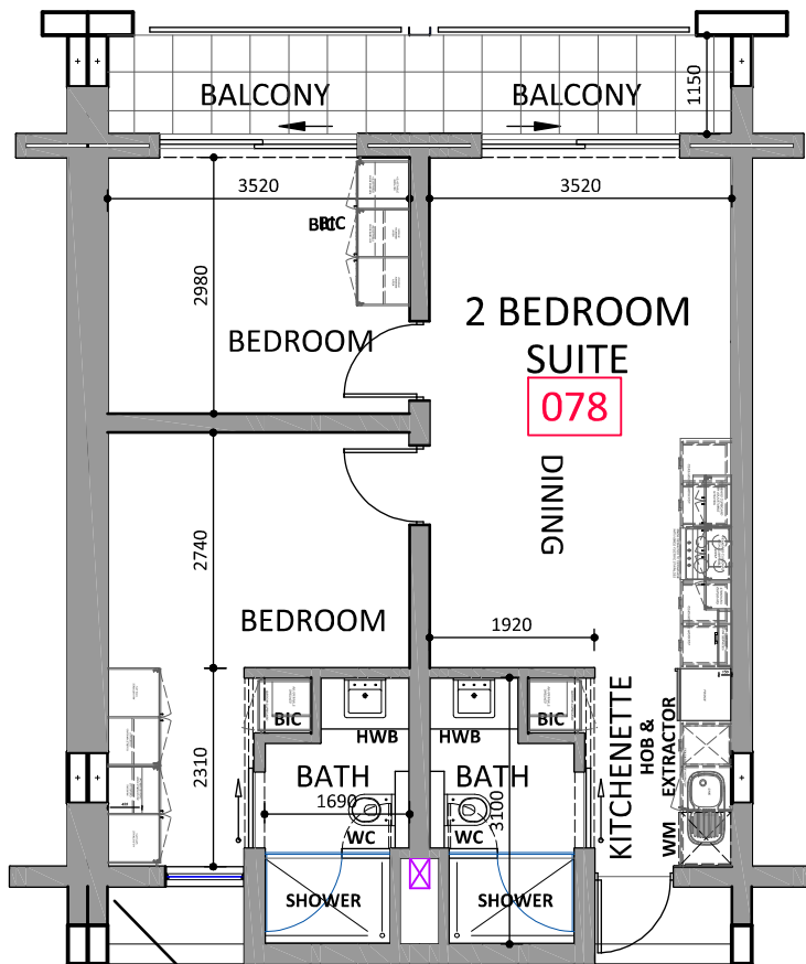
UNIT 078 SECOND PLAN LAYOUT - Scale 1:100
