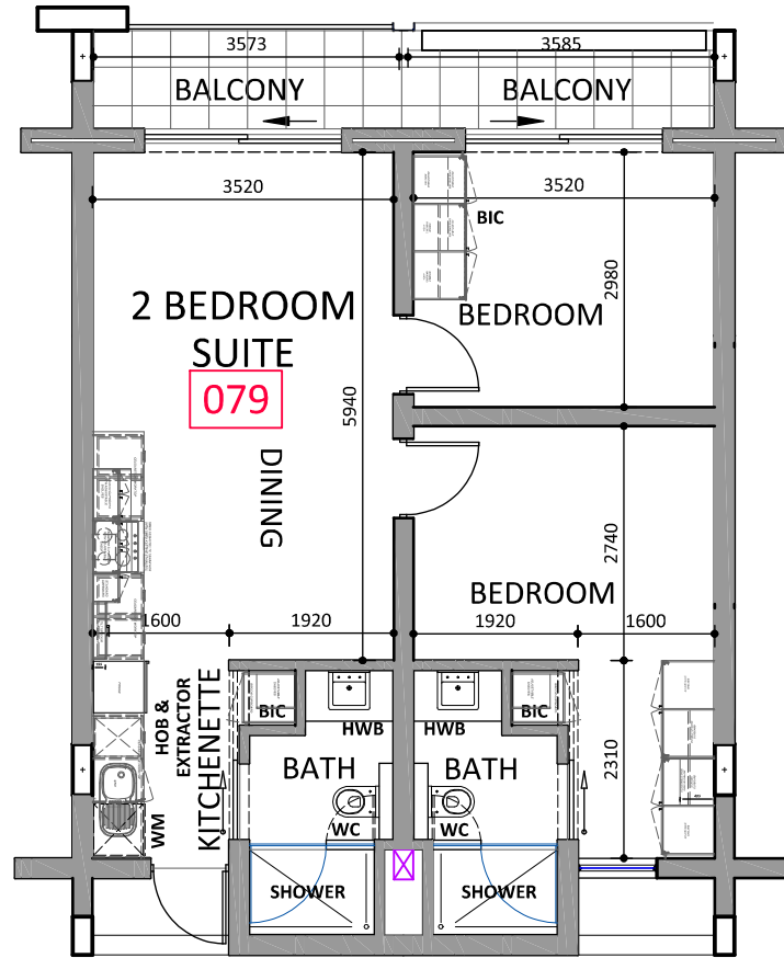
UNIT 079 SECOND PLAN LAYOUT - Scale 1:100
