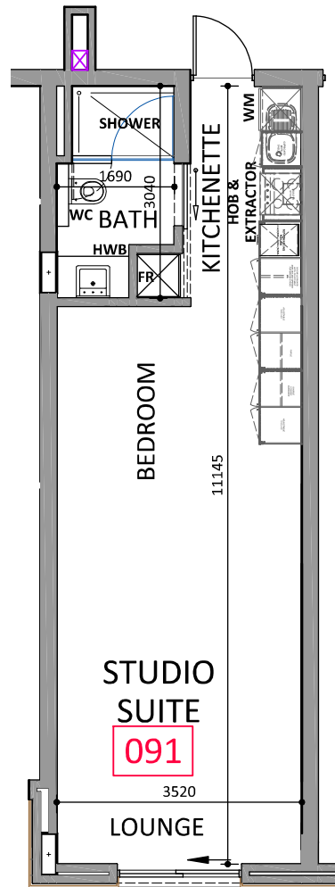
UNIT 091 SECOND PLAN LAYOUT - Scale 1:100
