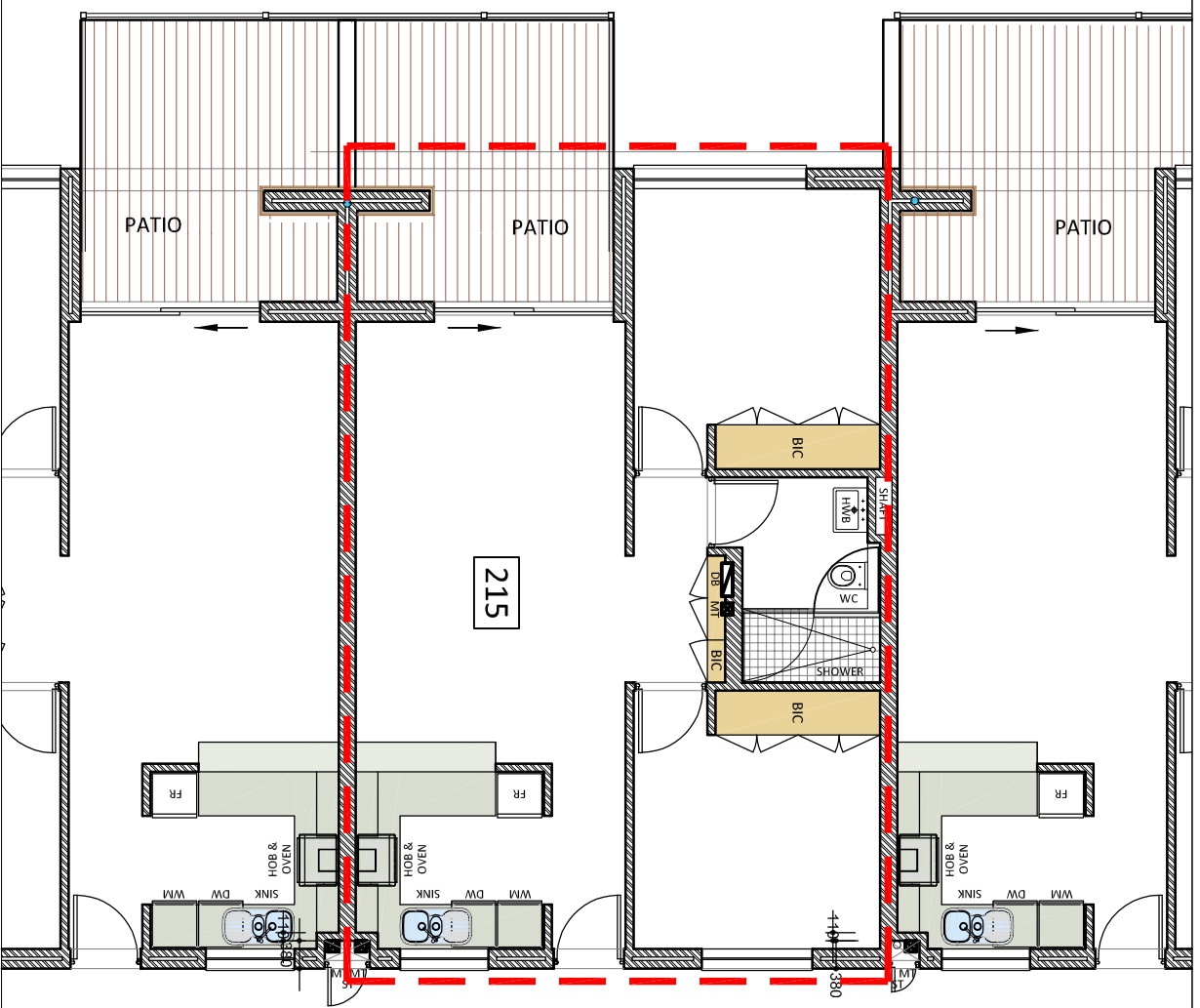
UNIT FLOOR PLAN LAYOUT - Scale 1:100
