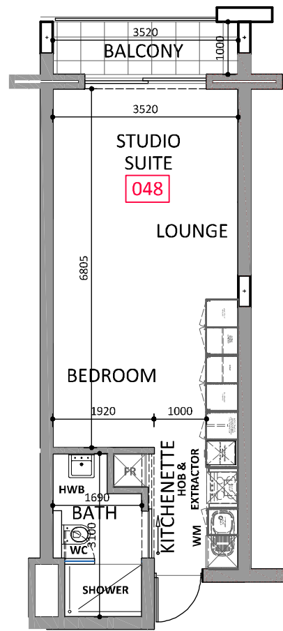
UNIT 048 FIRST PLAN LAYOUT - Scale 1:100
