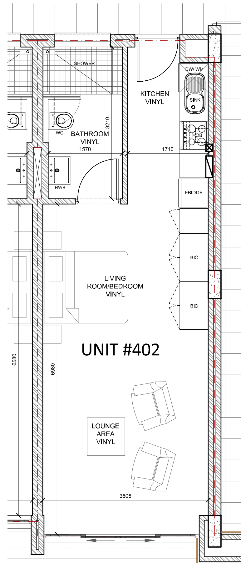
GROUND FLOOR - UNIT 402 SCALE 1:50
