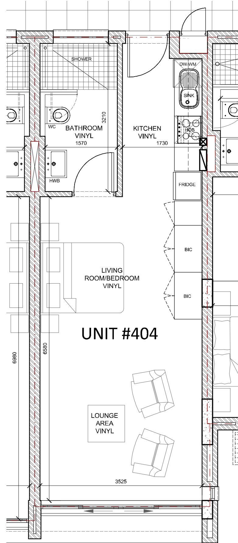
GROUND FLOOR - UNIT 404 SCALE 1:50
