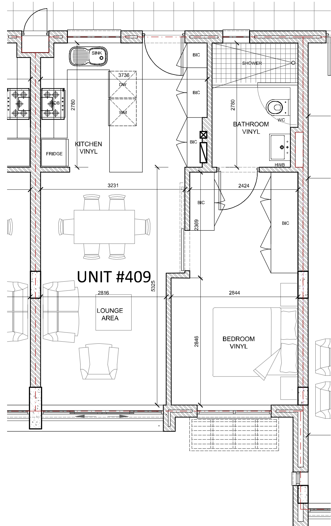
GROUND FLOOR - UNIT 409 SCALE 1:50
