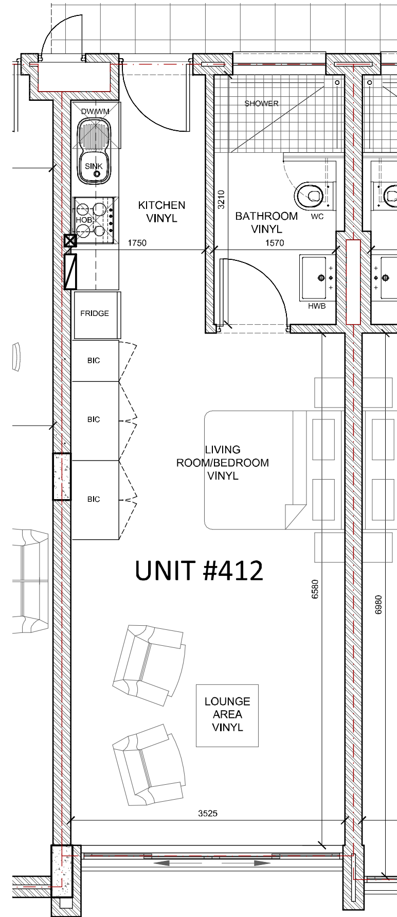
FIRST FLOOR - UNIT 412 SCALE 1:50
