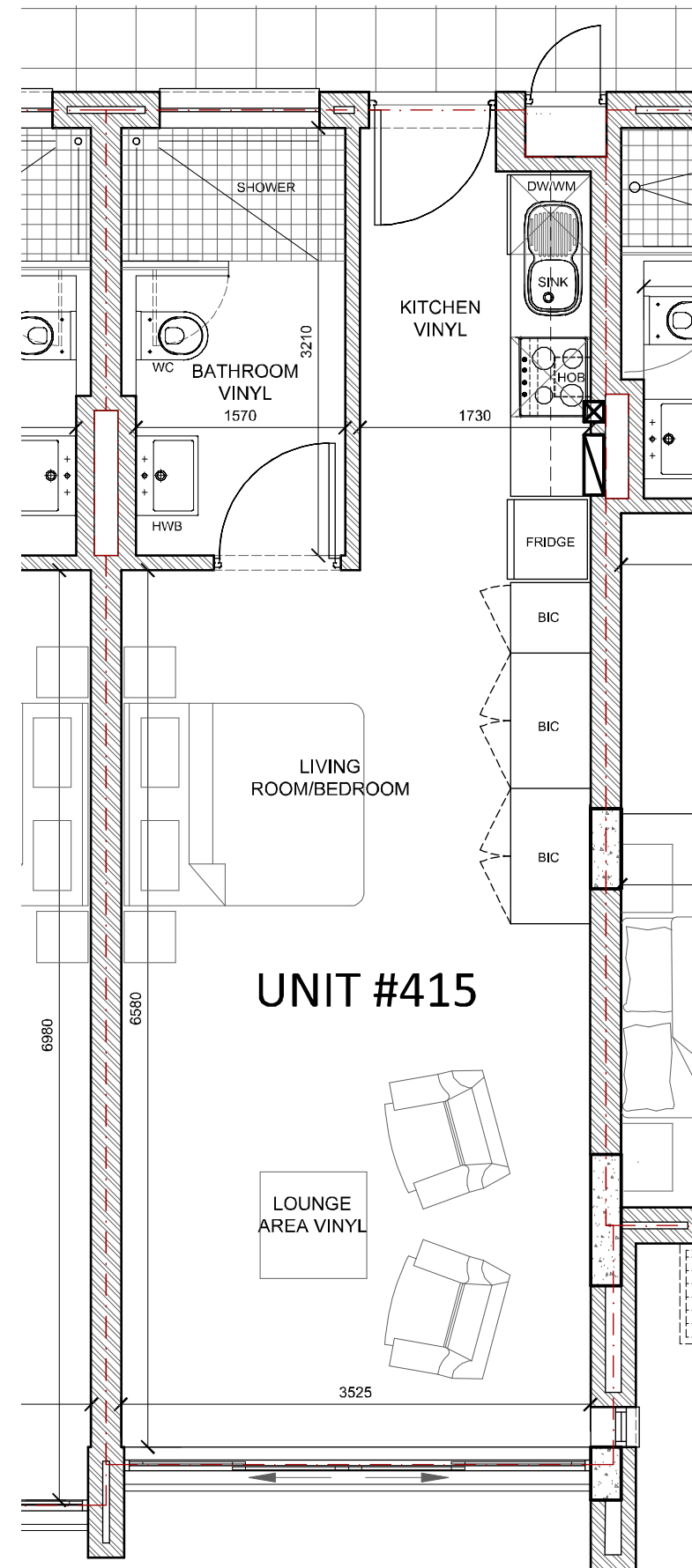
FIRST FLOOR - UNIT 415 SCALE 1:50
