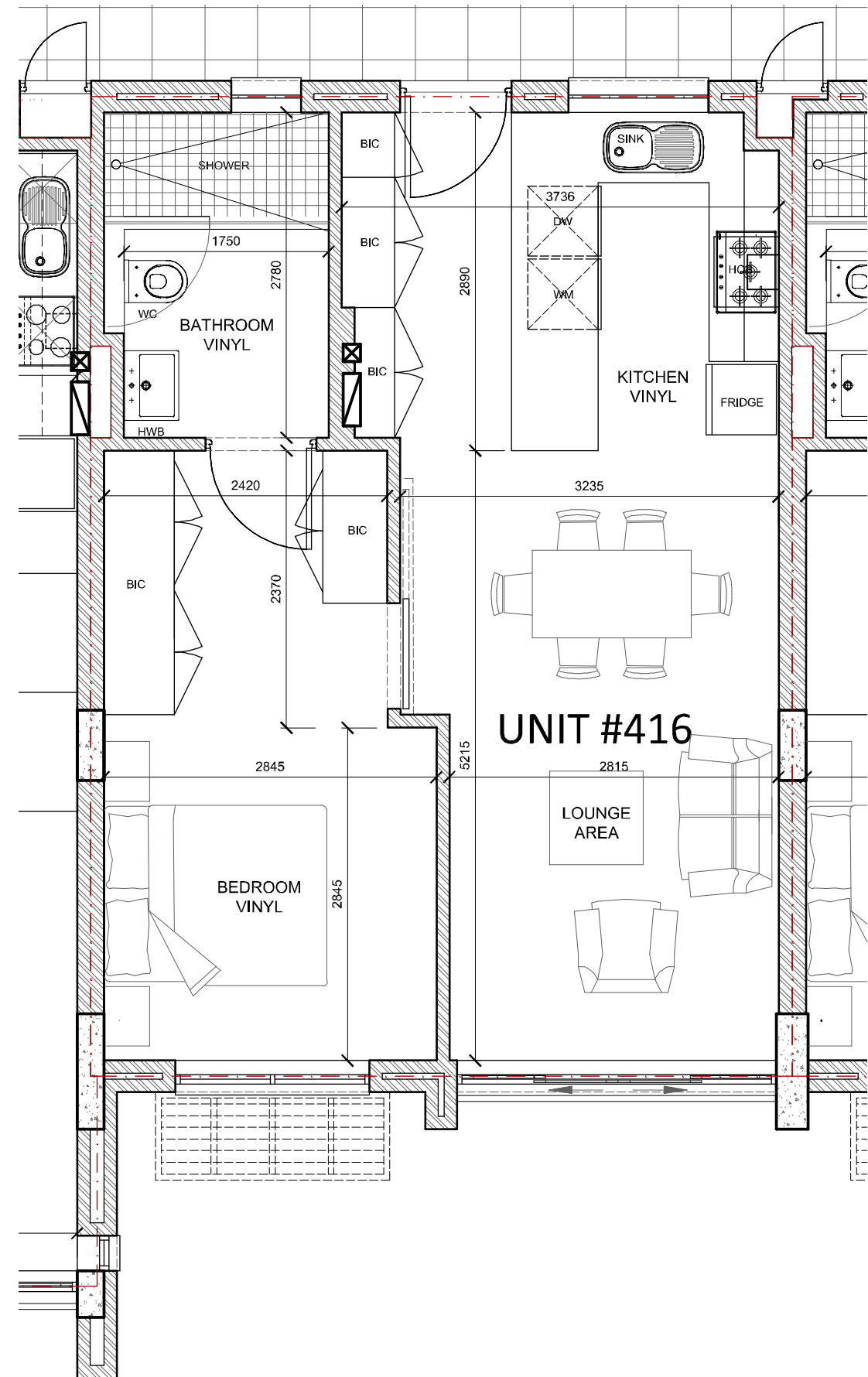
FIRST FLOOR - UNIT 416 SCALE 1:50
