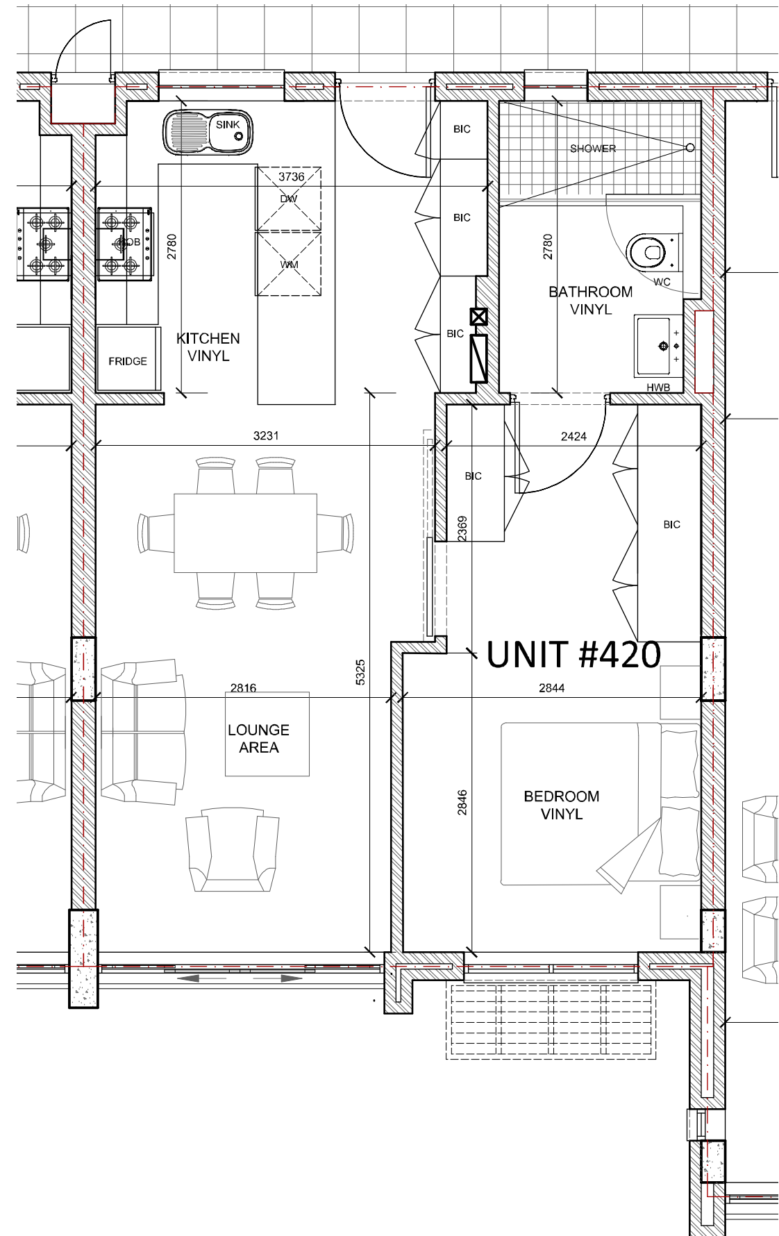
FIRST FLOOR - UNIT 420 SCALE 1:50
